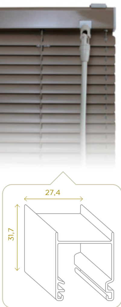
Rail SG 10037 SG 10037 track
