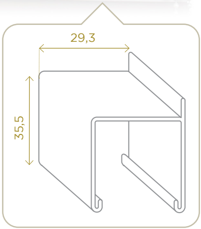
Rail SG 8301 SG 8301 track
