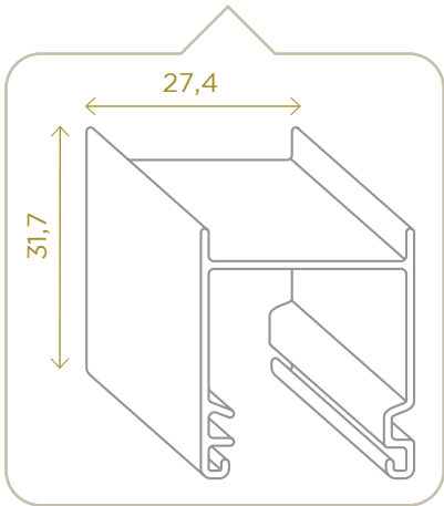
Rail SG 10037 SG 10037 track
