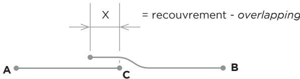
C6 - Cintrage en S ou overlap. Vue de dessus. - Overlap bending. Top view.
