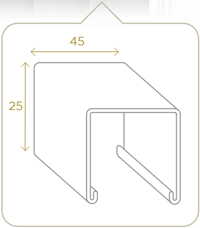
Rail métallique Head rail
