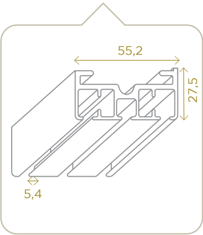
Profil SG 5300 SG 5300 track profile
