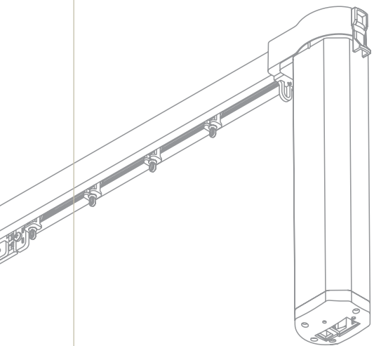
Profil SG 5100 monté Mounted SG 5100 track
