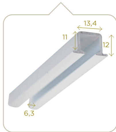
Profil rail 6243 6243 track profile
