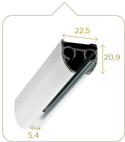
Profil rail 3841 3841 track profile
