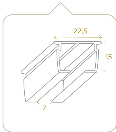
Profil rail 15x22.5 15x22.5 track profile
