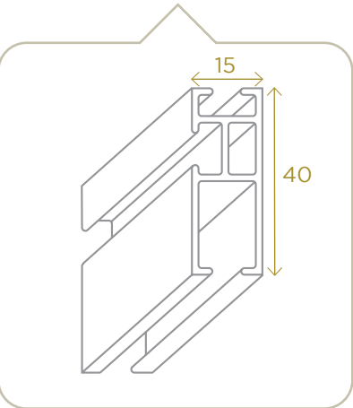
Profil 40x15 40x15 track profile
