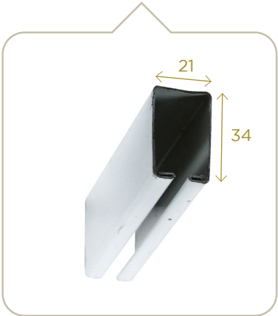
Profil rail 35x20 35x20 track profile
