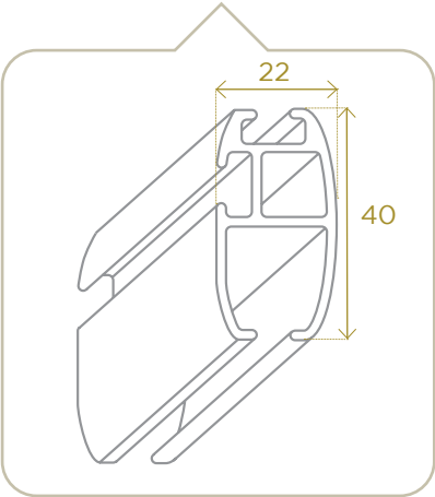
Profil 40x22 40x22 track profile
