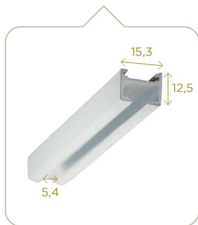
Profil rail 6465 6465 track profile
