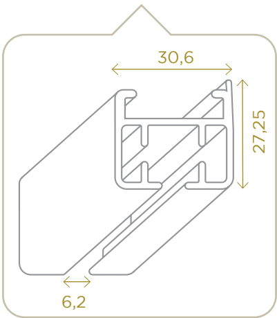
Profil SG 5100 SG 5100 track profile
