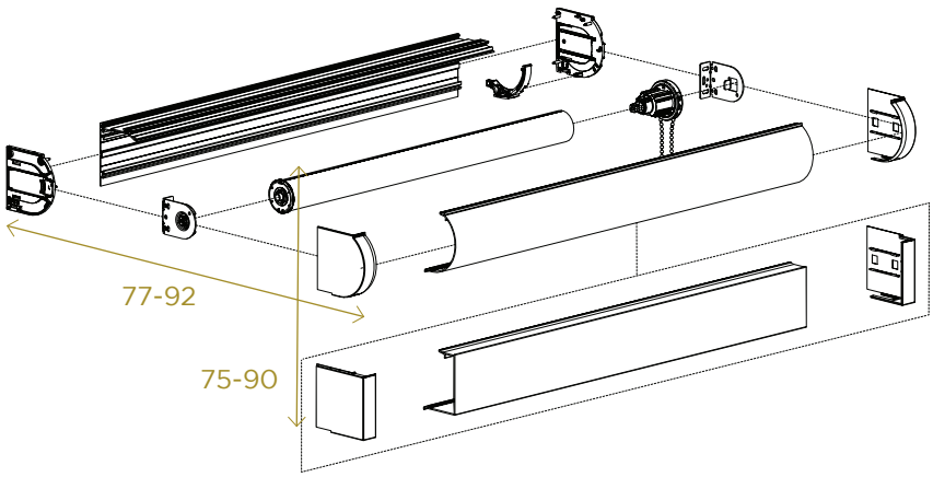
Façade Fascia
